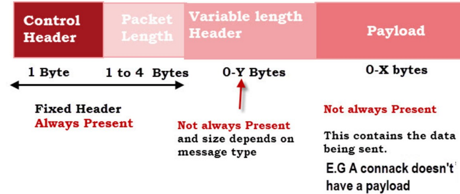
MQTT Standard Packet Structure
