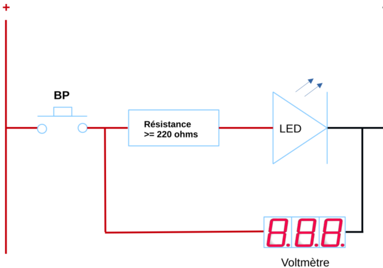
BP inter double LED RVB Cathode commune
