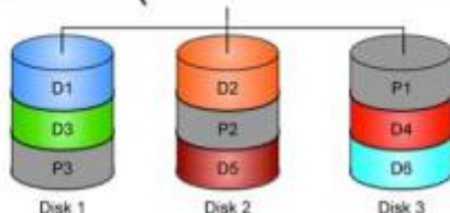
RAID 5 (Drives with Parity)
